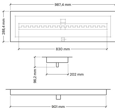
SINGLE BURNER
