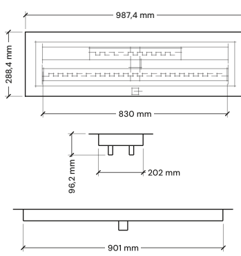
SPLIT LINE
